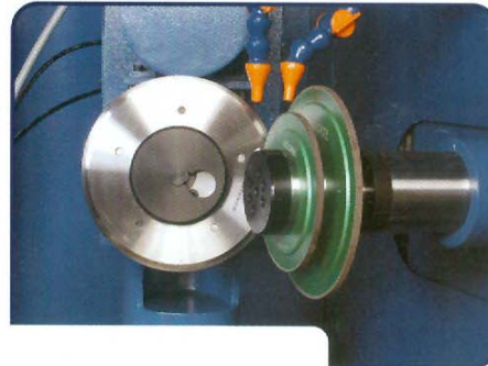
Roughing and finishing in one operation.
