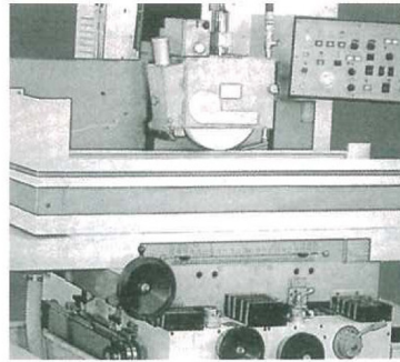
Surface Grinding Wheels Horizontal Spindle Type
